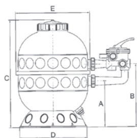
Dimensions of HI Side filter
